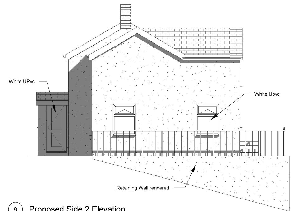
6 Proposed Side 2 Elevation 1 : 100
