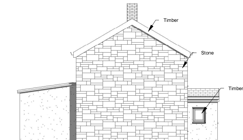
5 Existing Side 1 Elevation 1 : 100
