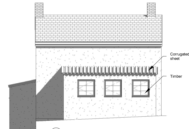
4 Existing Rear Elevation 1 : 100
