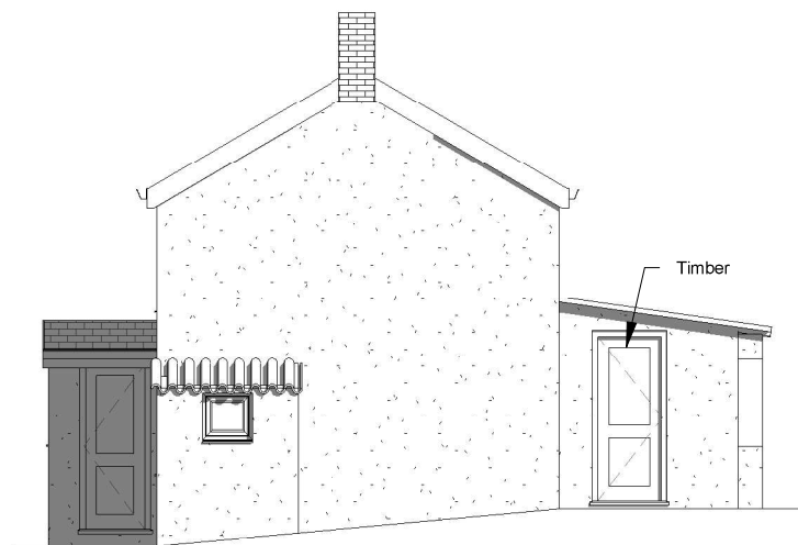
6 Existing Side 2 Elevation 1 : 100
