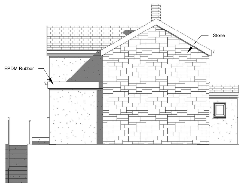
5 Proposed Side 1 Elevation 1 : 100
