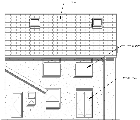
2 Existing Rear Elevation 1 : 100
