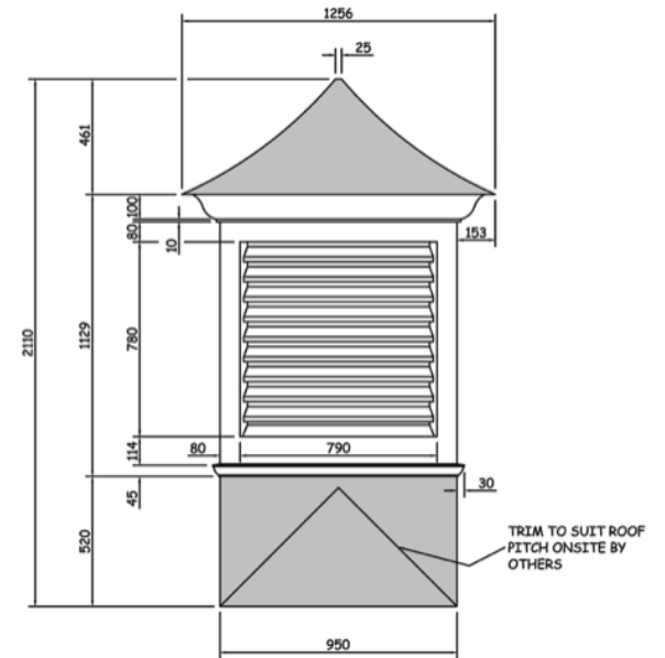
Cupola- timber with lead roof
