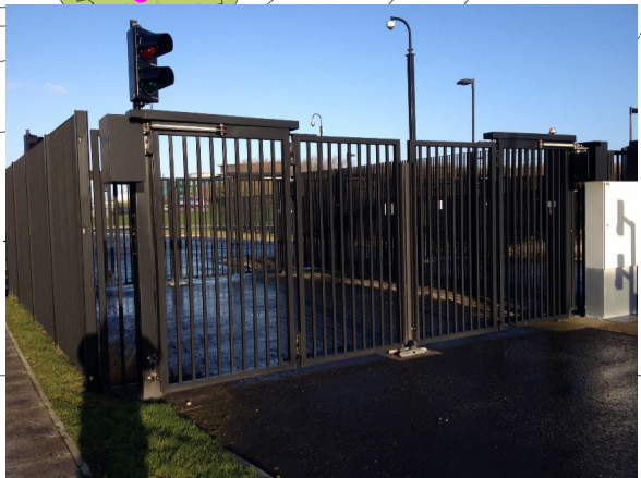
Vertical Bar Railings & Post B-Folding Gates polyester powder coated (Colour: Black)
