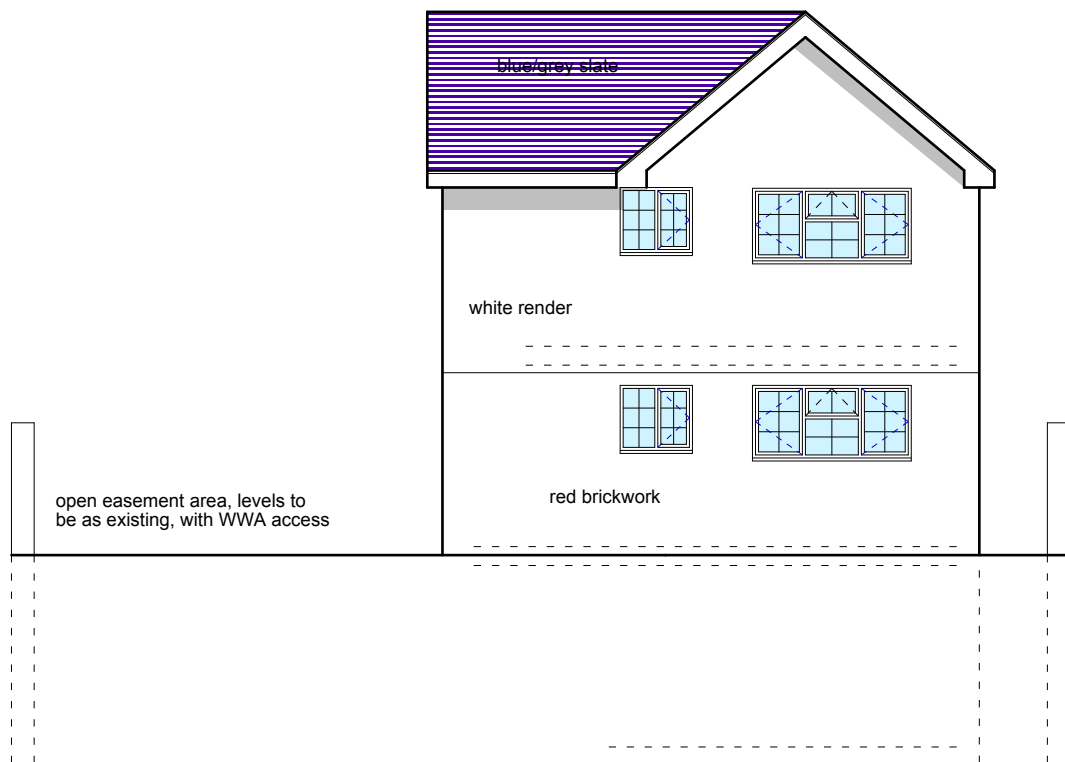
rear elevation
