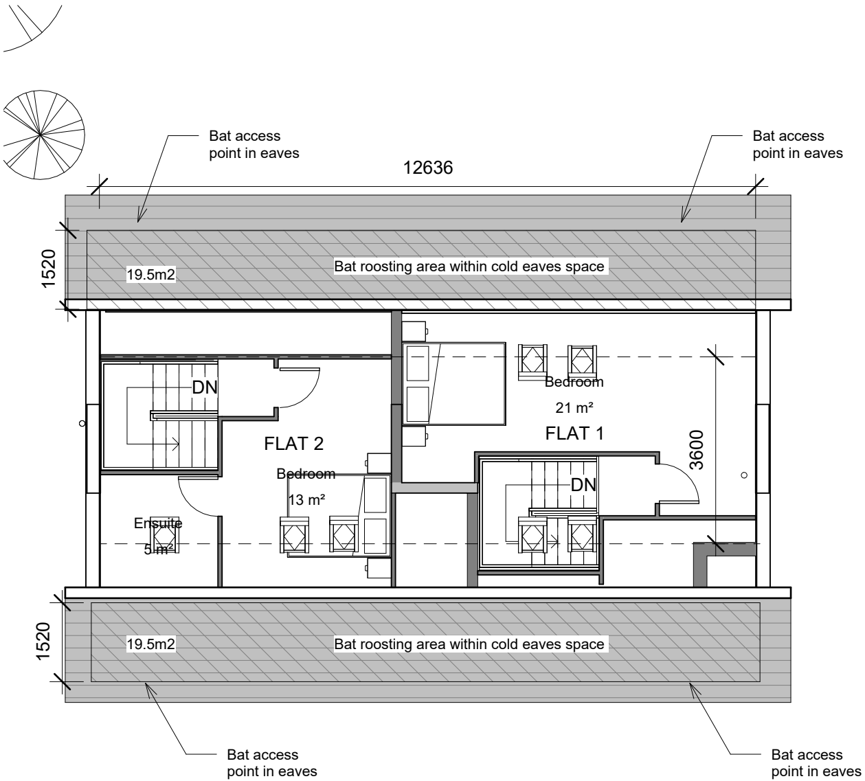
Proposed First Floor ( 1 : 100)
