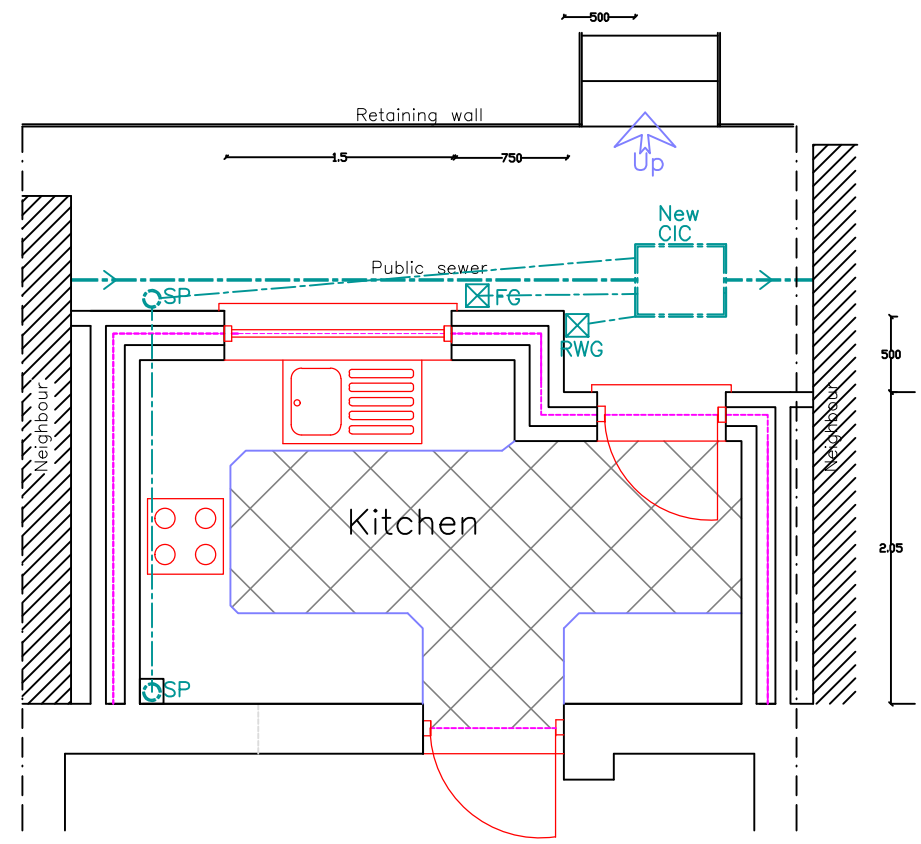
Proposed Extension Ground Floor Plan 1:50
