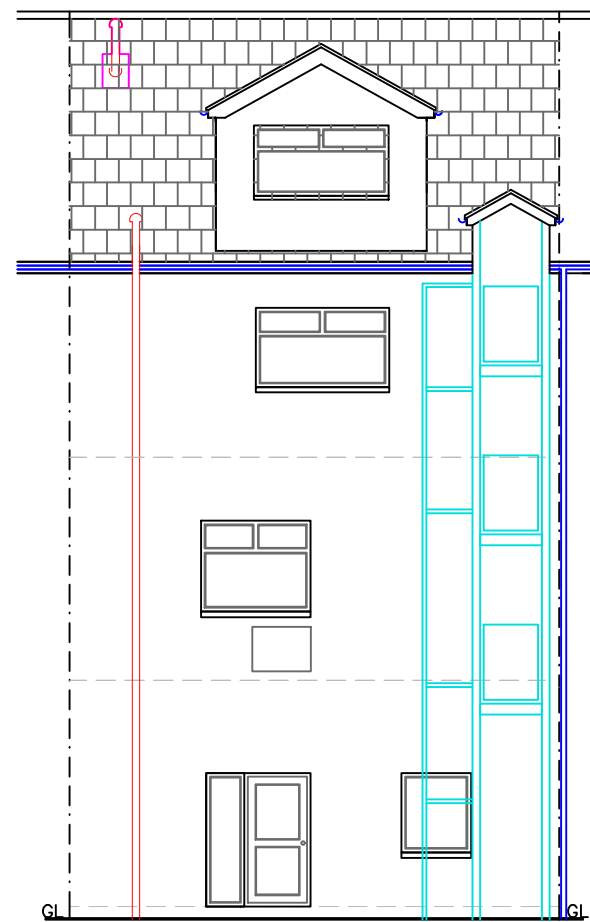
Proposed Rear Elevation 1:100 [No Change]
