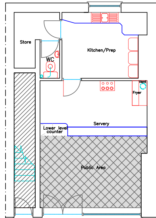
Proposed GF Plan 1:100
