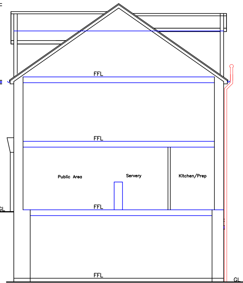
Proposed Section 1:100
