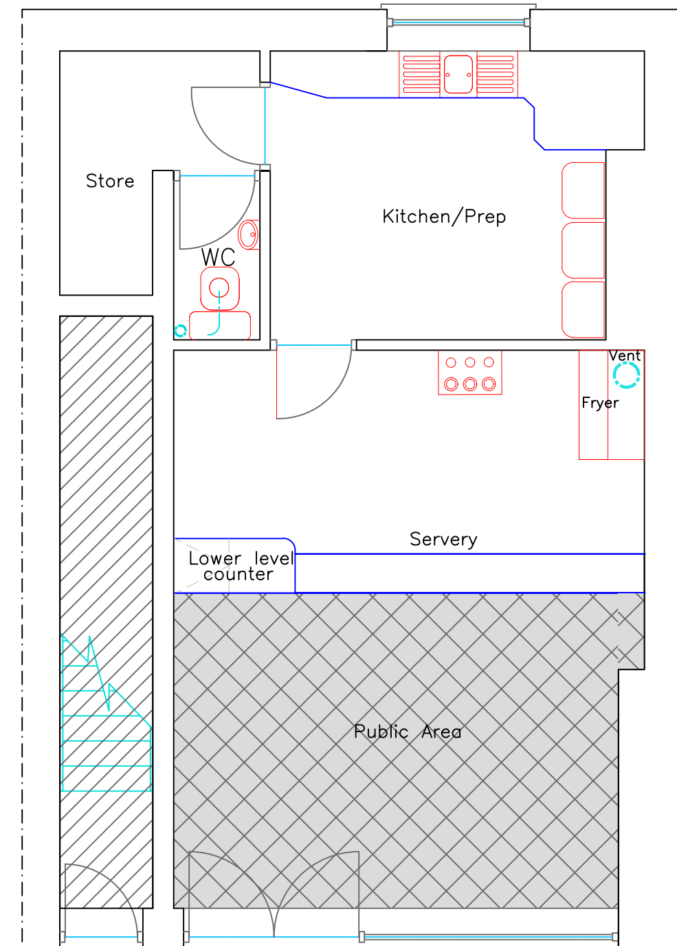
Proposed GF Plan 1:50
