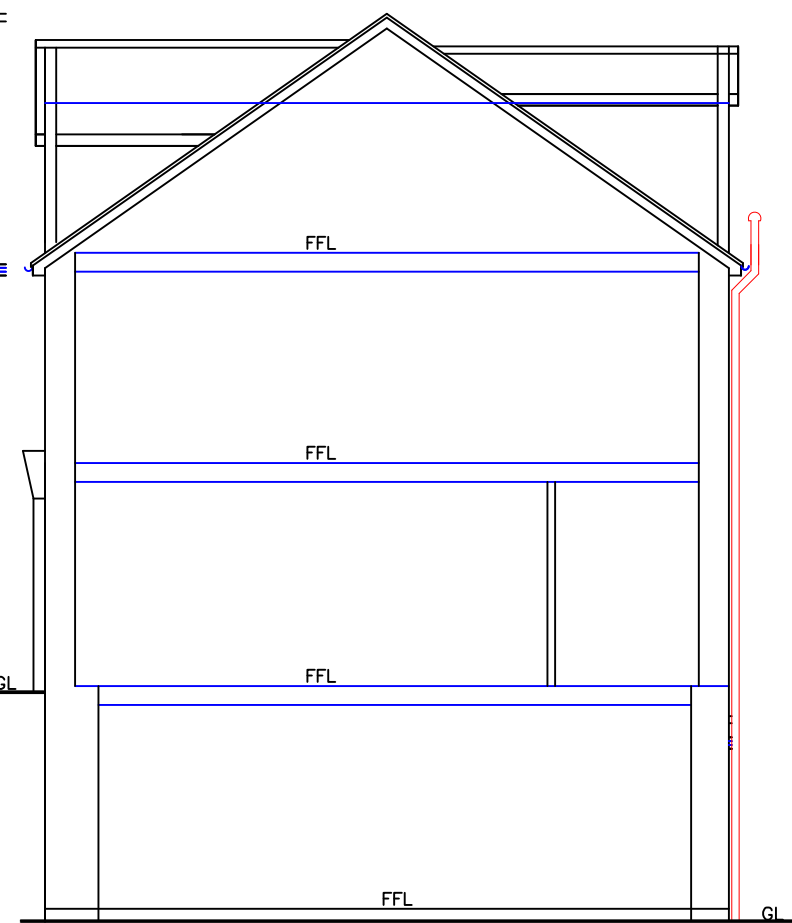
Existing Section 1:100
