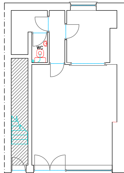
Existing GF Plan 1:100
