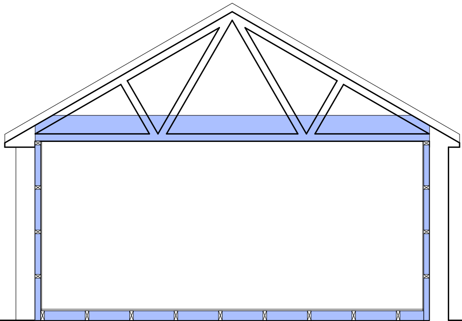
PROPOSED SECTION
