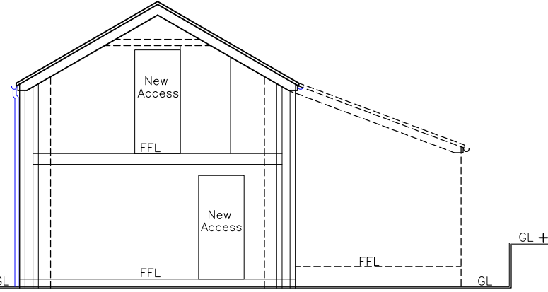
Proposed Extension Section 1:100
