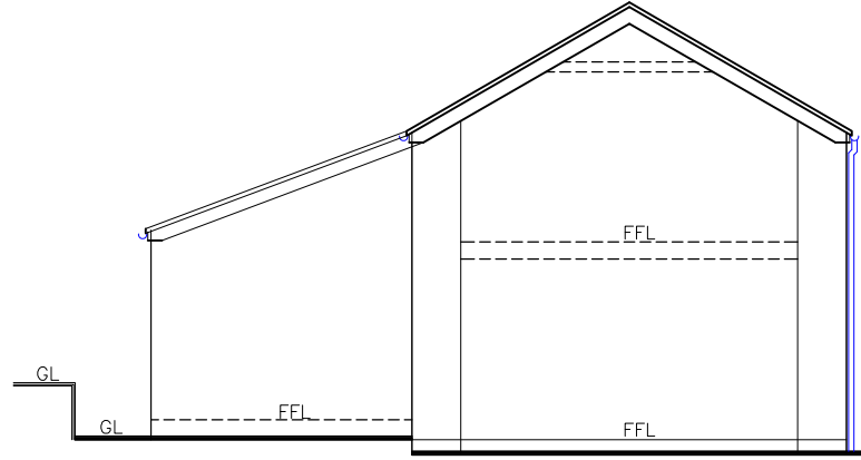
Existing House Section 1:100
