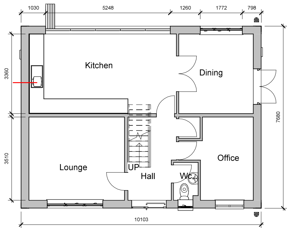
1 Ground Floor 1 : 100 1no Sparrow Box 1no intergrated bat block
