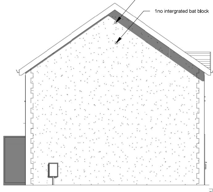
5 Side 1 Elevation 1 : 100
