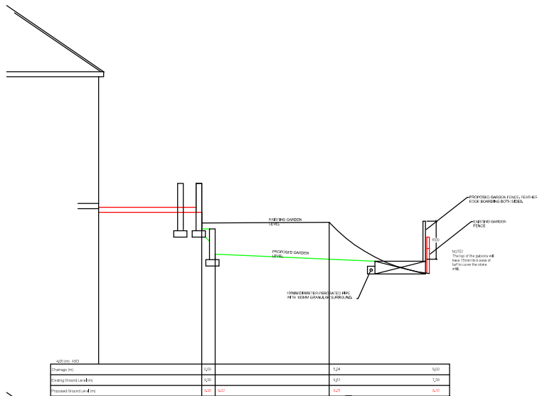
CROSS SECTION 4-4 (1:100)
