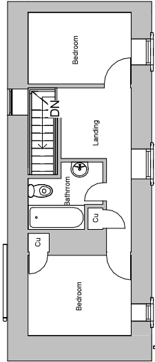
2 Proposed First Floor 1 : 100
