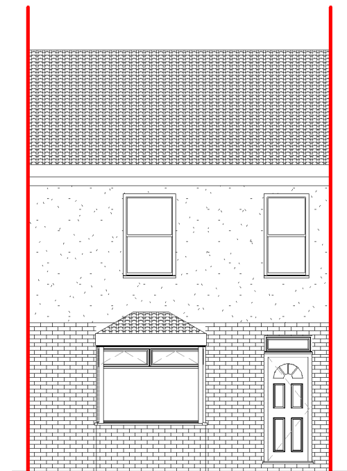
Front Elevation 1 : 100
