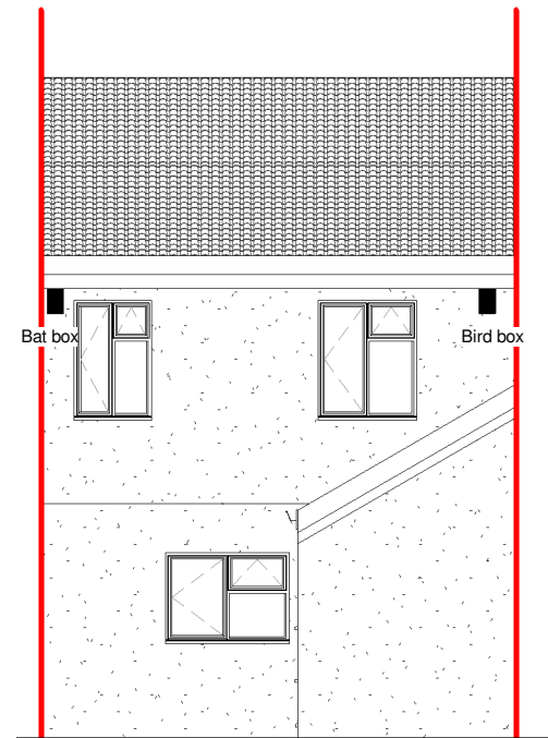
Rear Elevation 1 : 100
