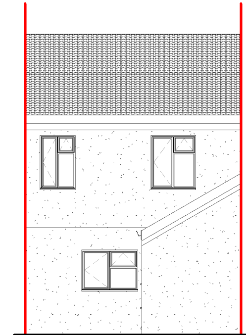
Rear Elevation 1 : 100
