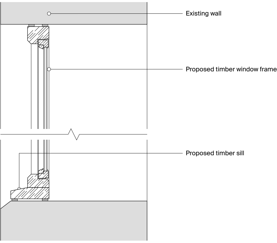
03 Head & sill - proposed section detail Scale: 1:10
