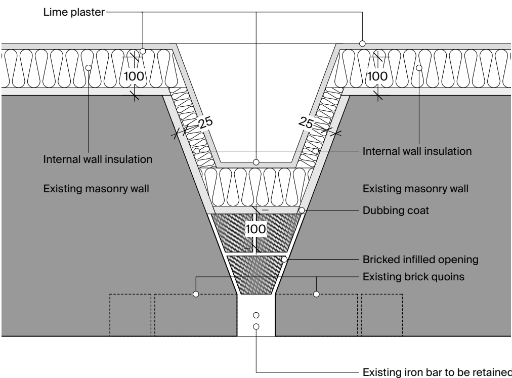
01 Threshing barn - slot window detail Scale: 1:10
