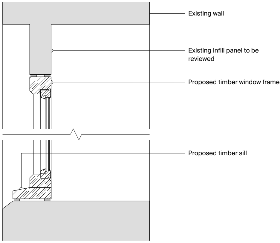
04 Head & sill - proposed section detail Scale: 1:10
