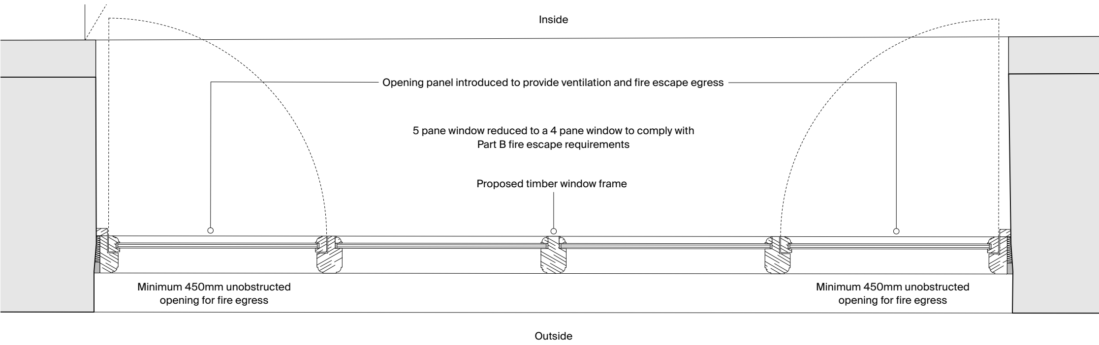
Proposed plan detail - replacement Scale: 1:10
