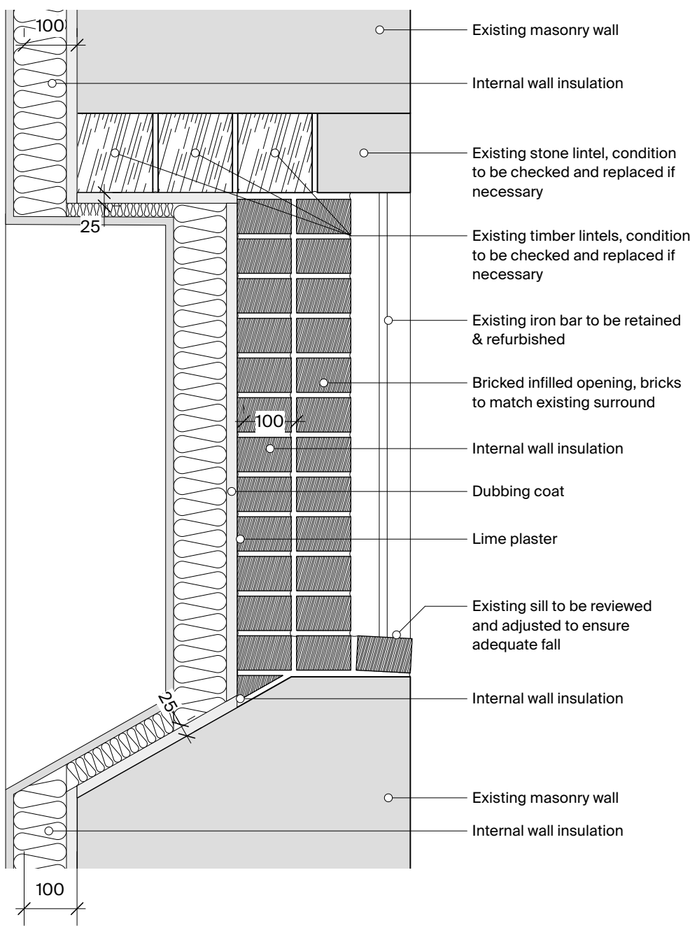
01 Threshing barn - slot window detail Scale: 1:10
