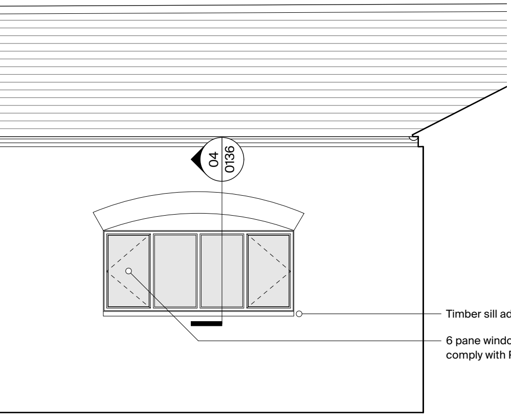
Typical window Scale: 1:100
