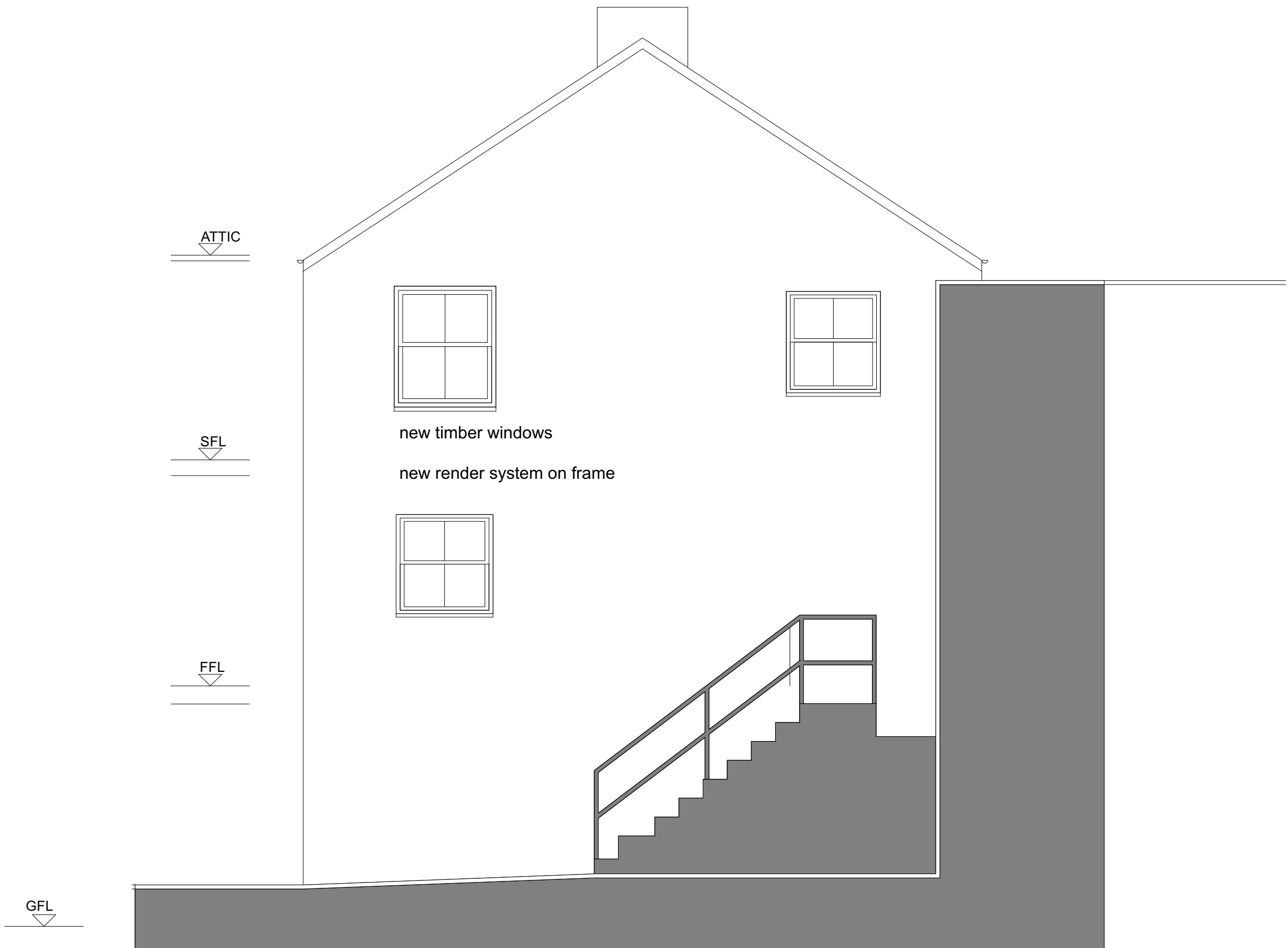
SIDE ELEVATION
