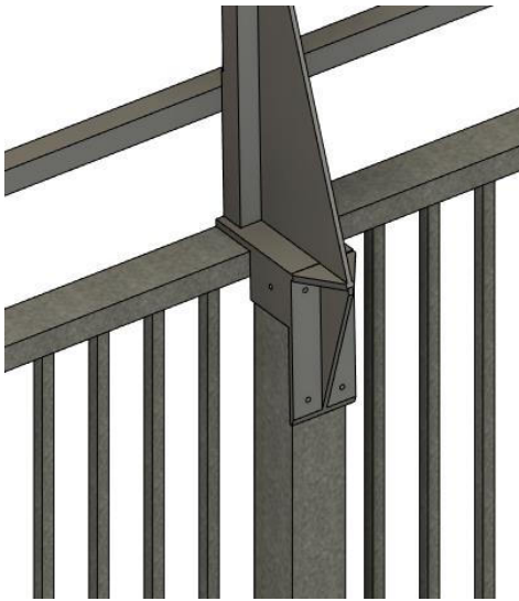
PART ILLUSTRATION OF BRACKETRY (REAR VIEW)
