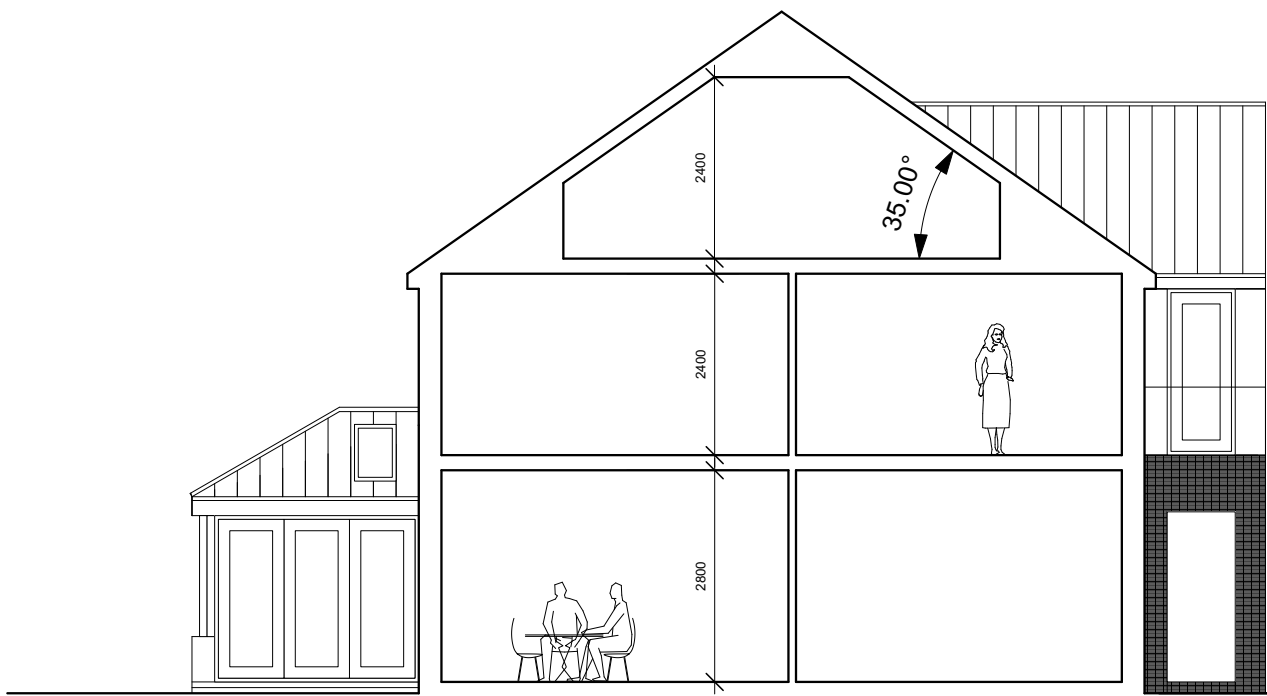
typical section
