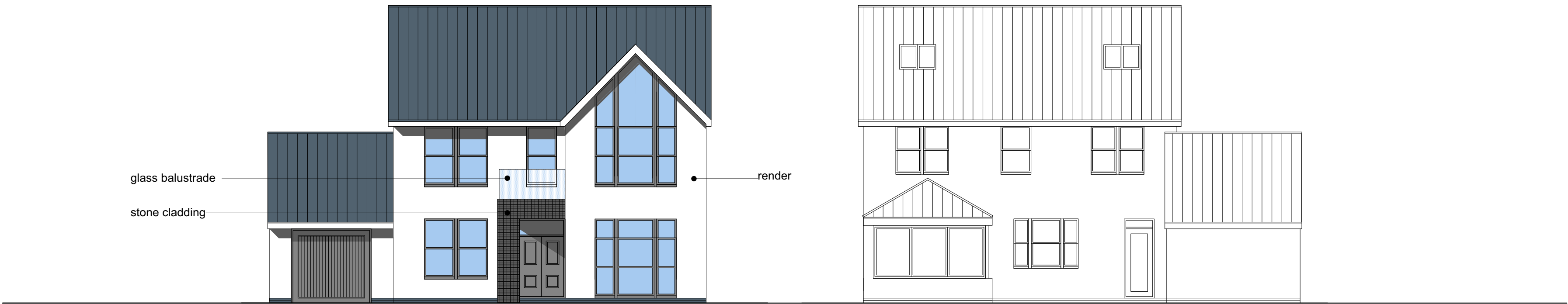
front elevation
