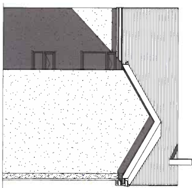
3 Proposed Rear Elevation 1 : 100
