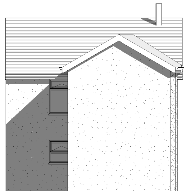
3 Proposed Rear Elevation 1 : 100
