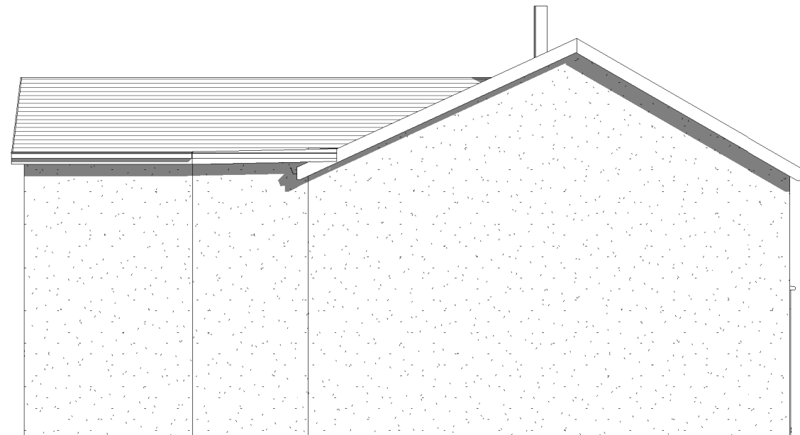
2 Proposed Side 1 Elevation 1 : 100
