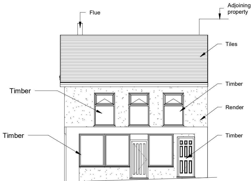
1 Proposed Front Elevation 1 : 100
