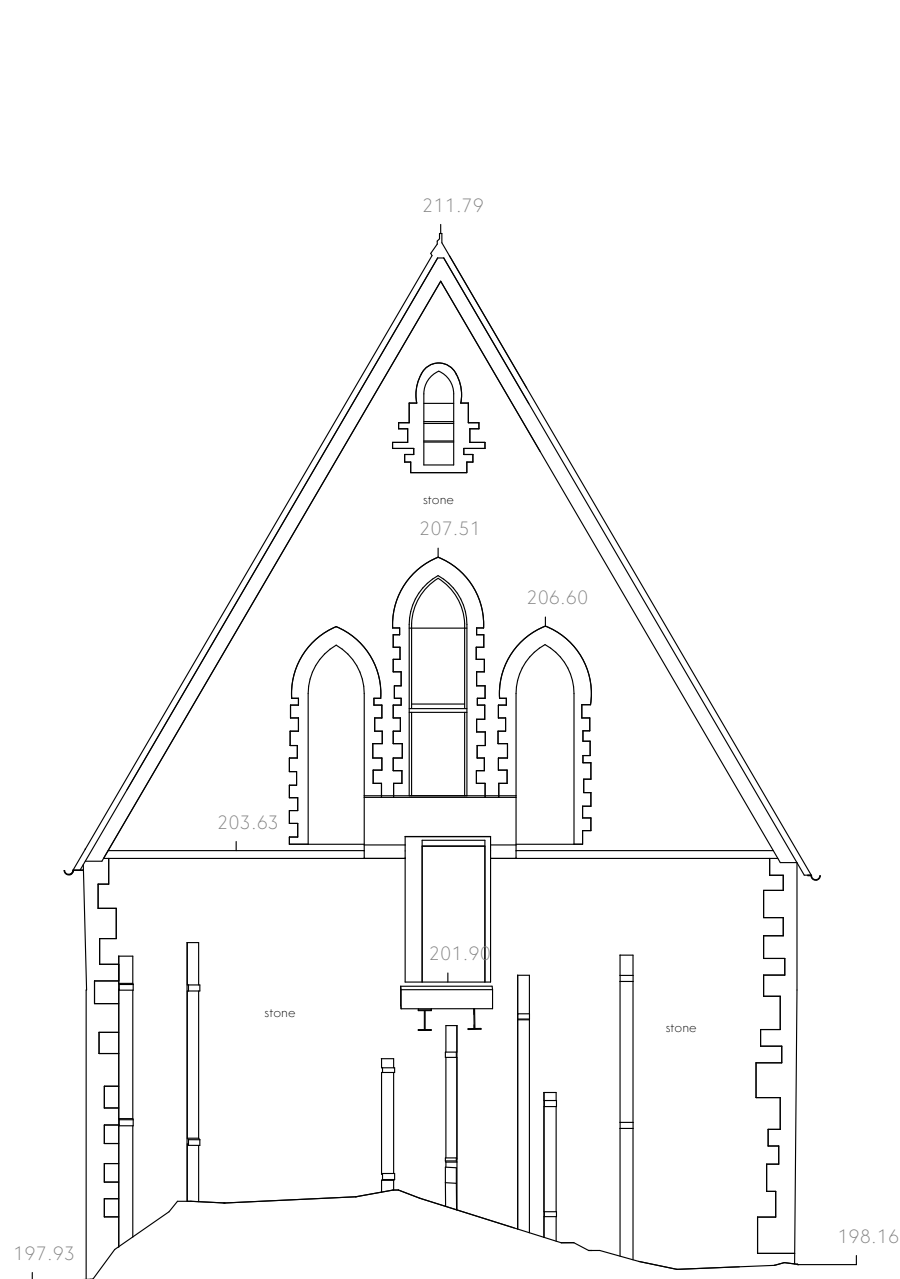
East Elevation
