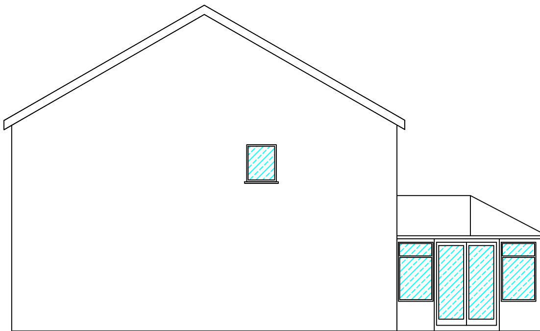
EAST SIDE ELEVATION PROPOSED
