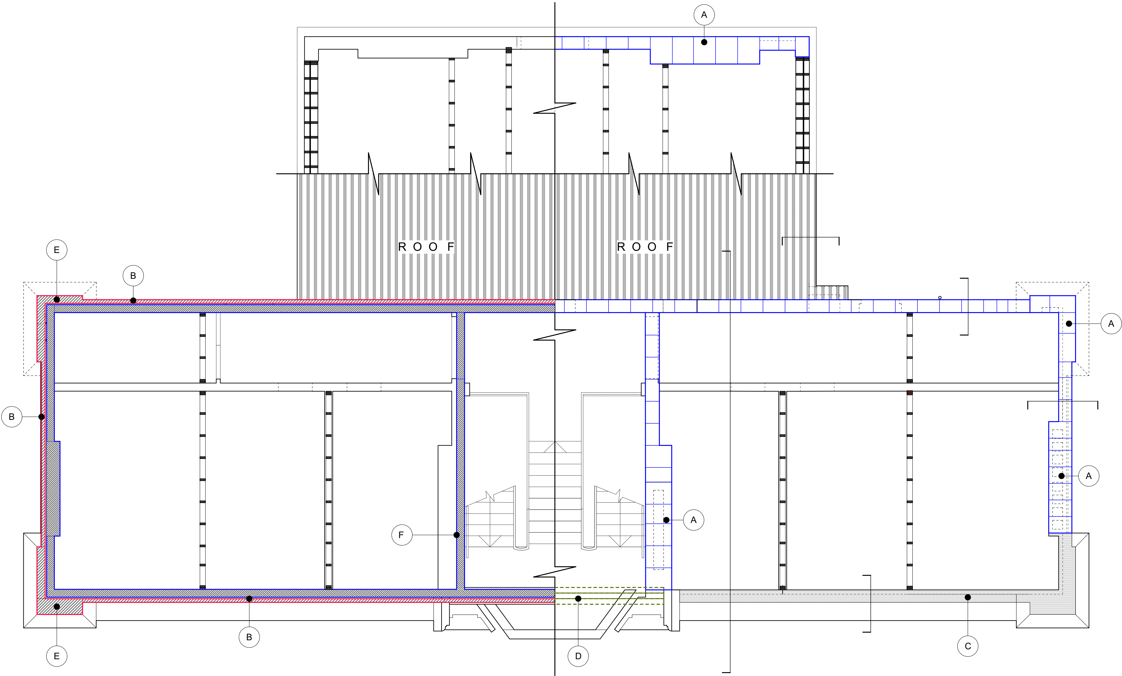
1 Proposed New High Level Masonry Plan, Above Capping Scale: 1:50
