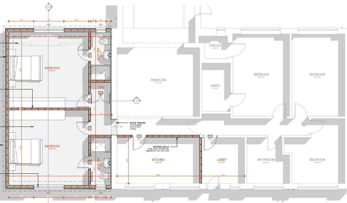
4 PROPOSED GROUND FLOOR 1:50
