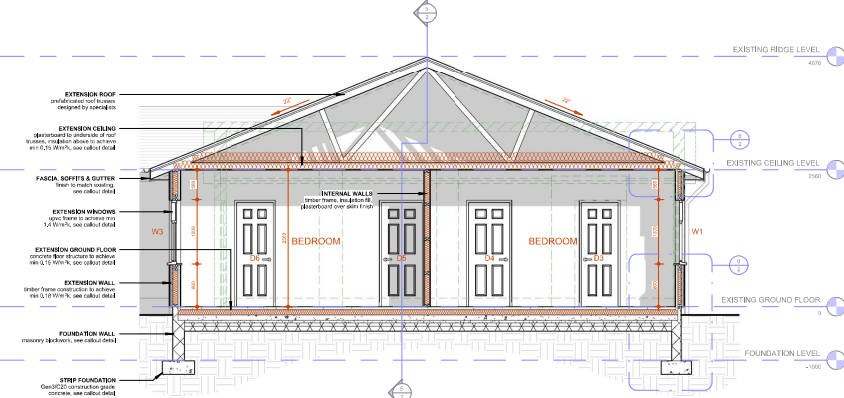
6 EXISTING LONG SECTION 1:50
