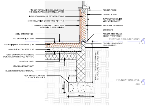
9 CALLOUT DETAIL 2 1:20
