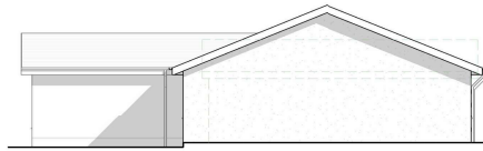
2 PROPOSED SIDE ELEVATION 1:100
