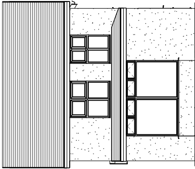
1 Proposed Front Elevation 1 : 100
