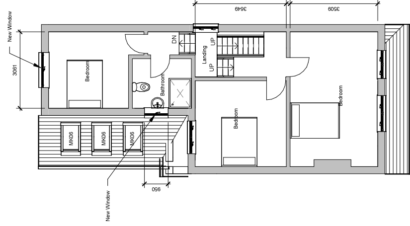
2 Proposed First Floor 1 : 100
