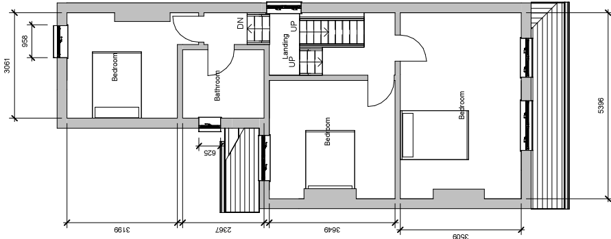
1 Existing First Floor 1 : 100
