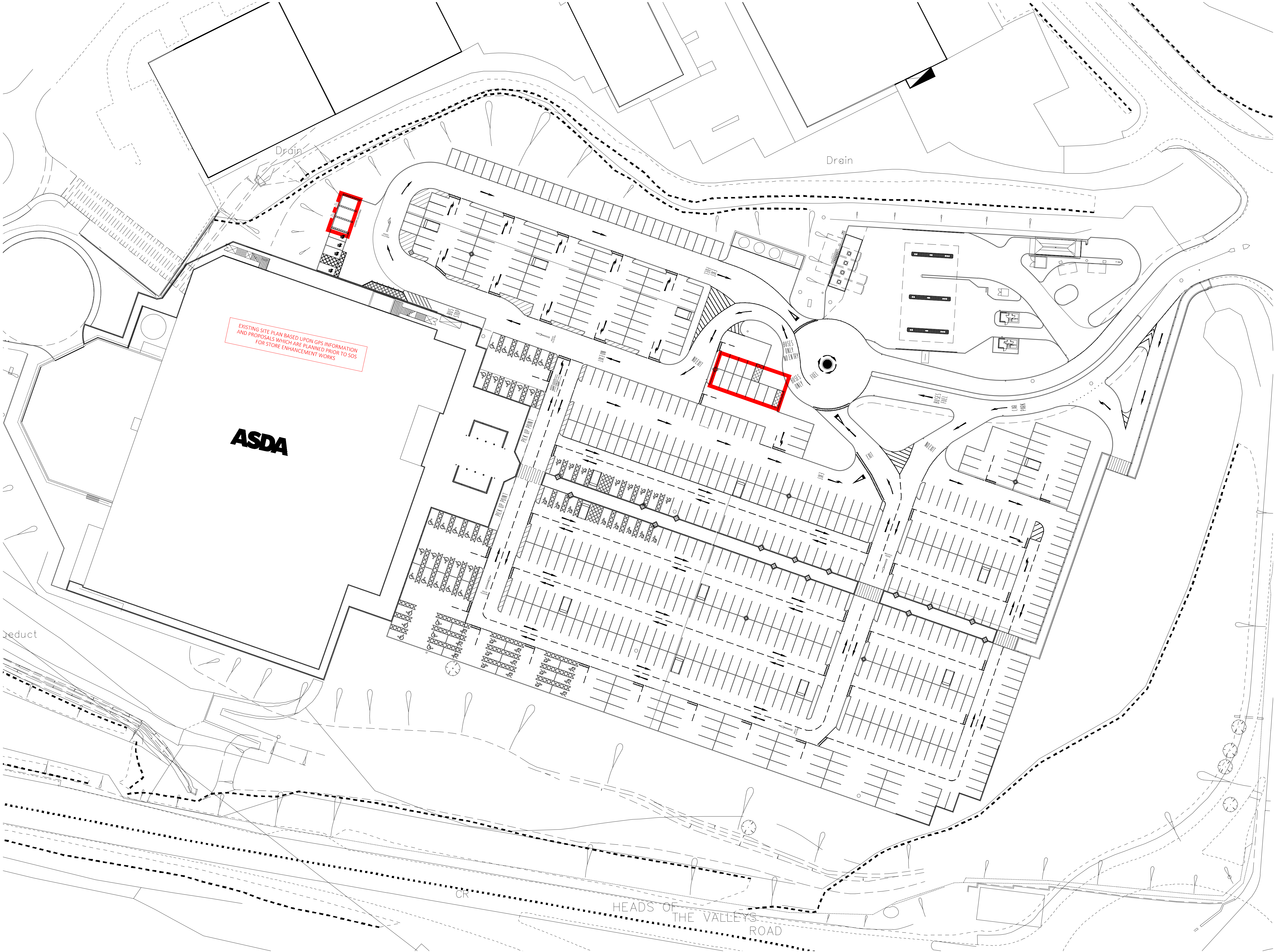
1 PROPOSED SITE LAYOUT PLAN PL-03 Scale 1:500 @ A1
