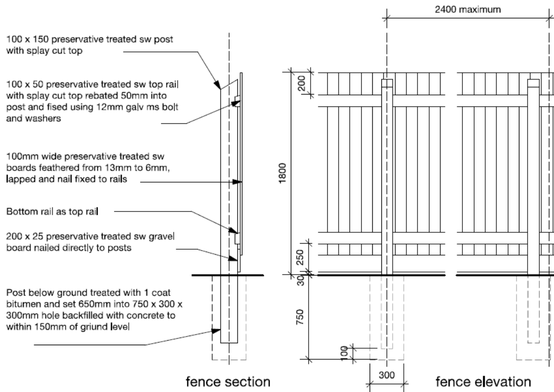
FENCE DETAIL 1:25
