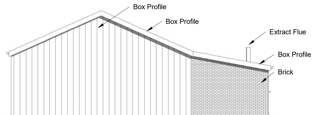
Proposed Side 2 Elevation
