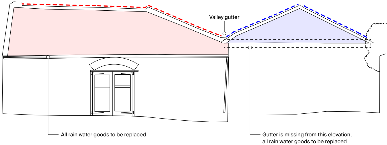
07 Existing elevation
