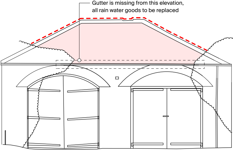
05 Existing elevation
