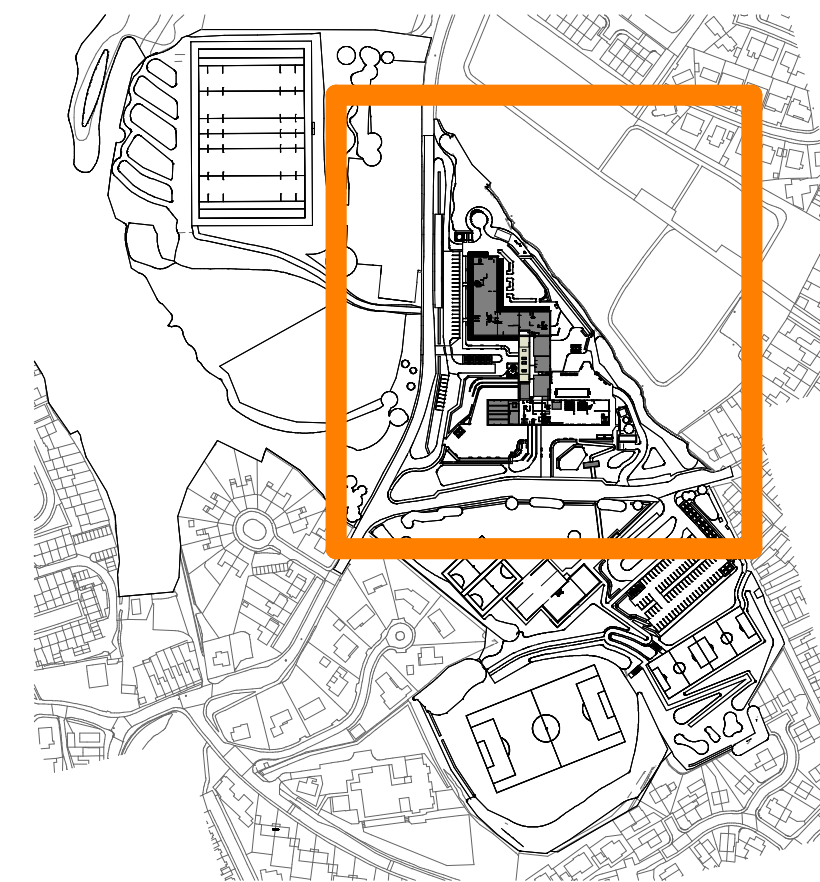
LOCATION PLAN 1:5000
