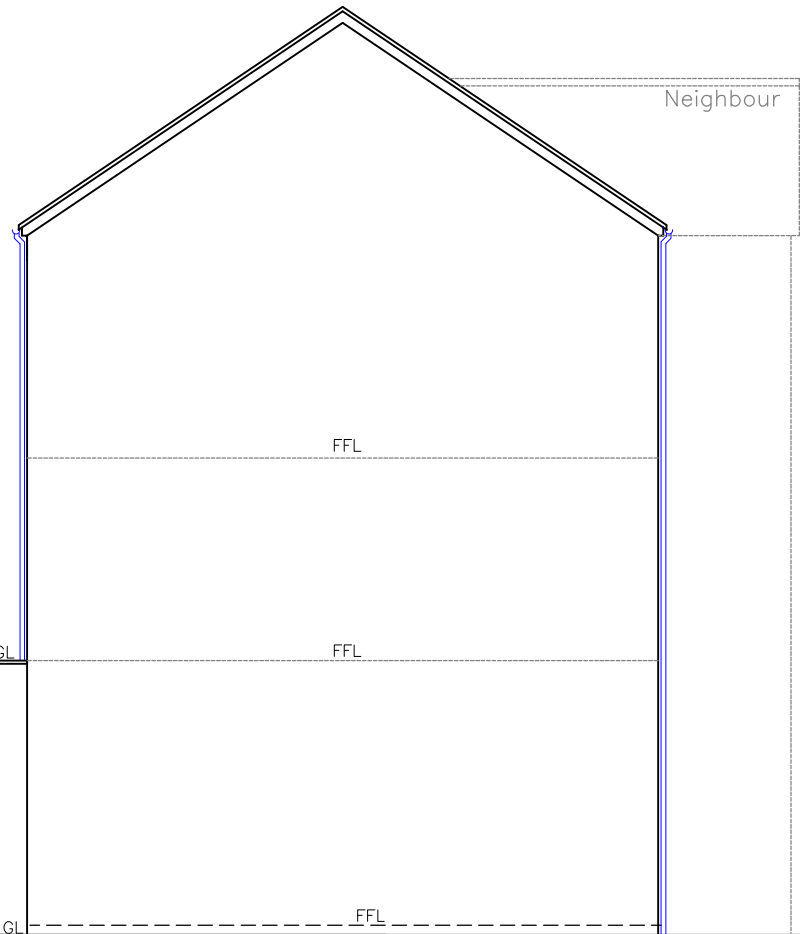
Proposed Side Elevation 1:100
