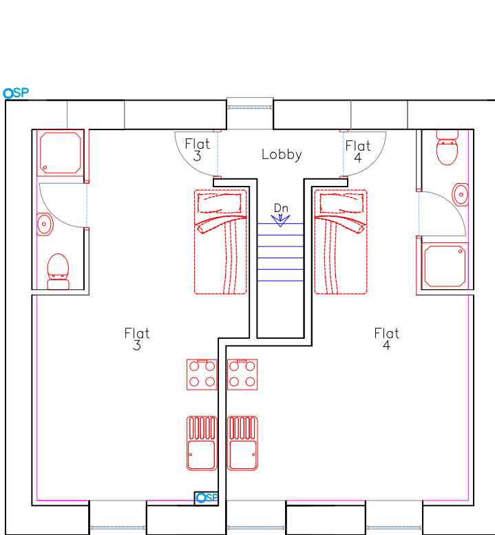
Proposed F Floor Plan 1:100
