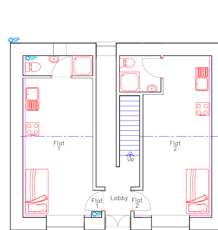
Proposed G Floor Plan 1:100
