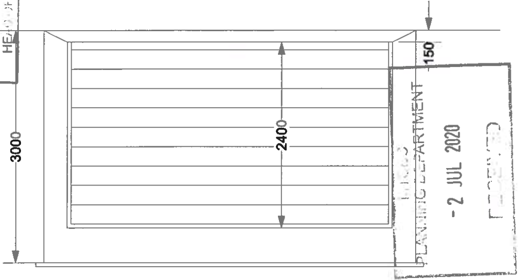
front elevation
