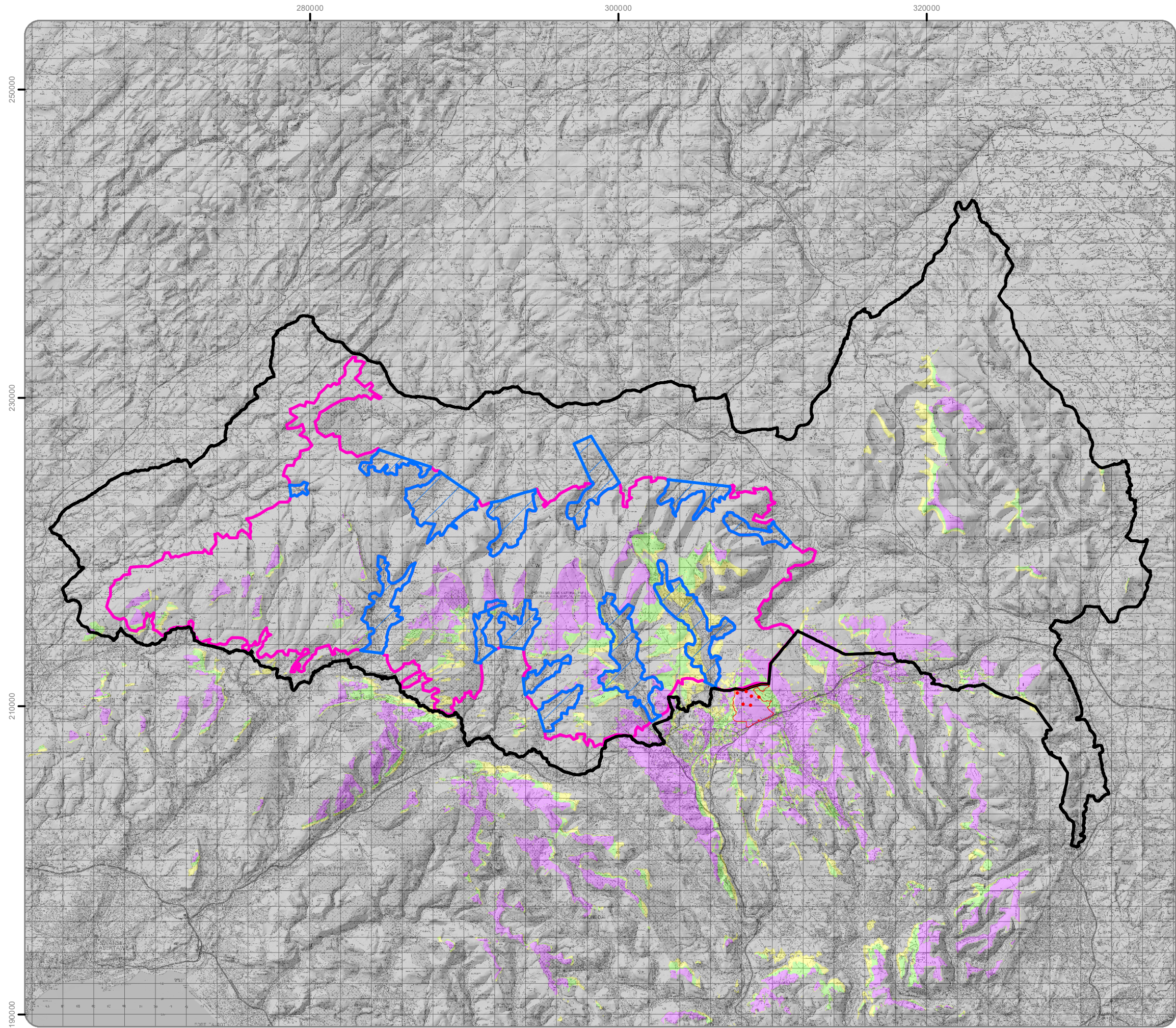
Figure TA5.5-5 ZTV of Turbine Tower Lighting (Dark Sky Reserve)
