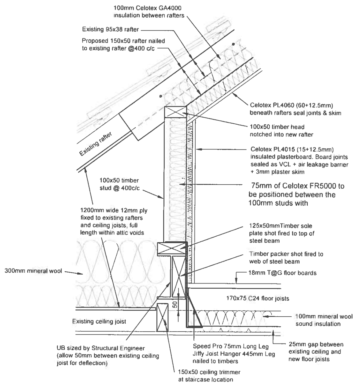
ATTIC SUPPORT - DETAIL 2
