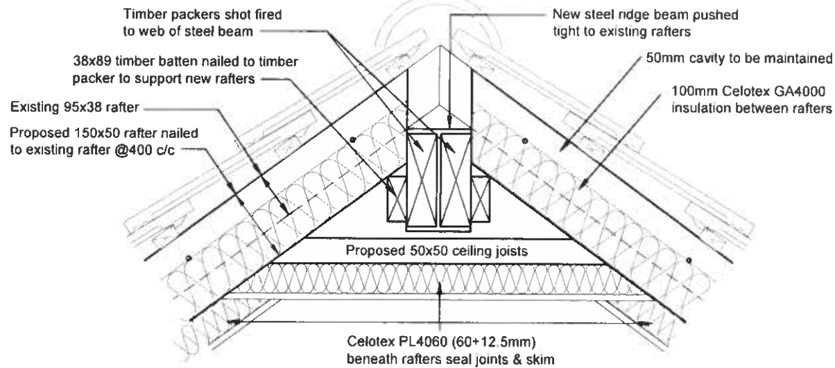
RIDGE - DETAIL 1
