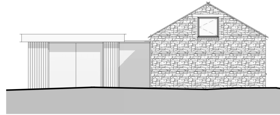
2 Proposed North West Elevation 1 : 100
