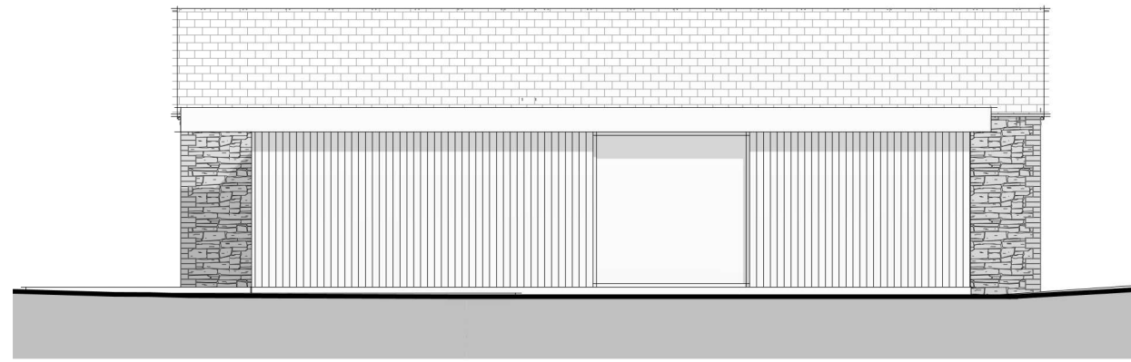
1 Proposed North East Elevation 1 : 100
