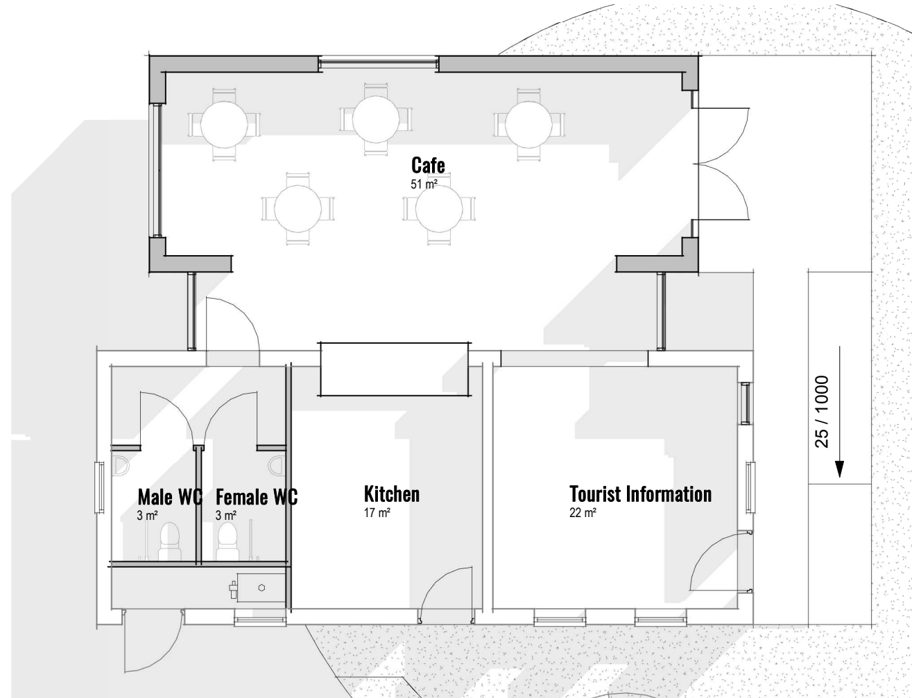
5 Proposed Ground Floor Plan 1 : 100
