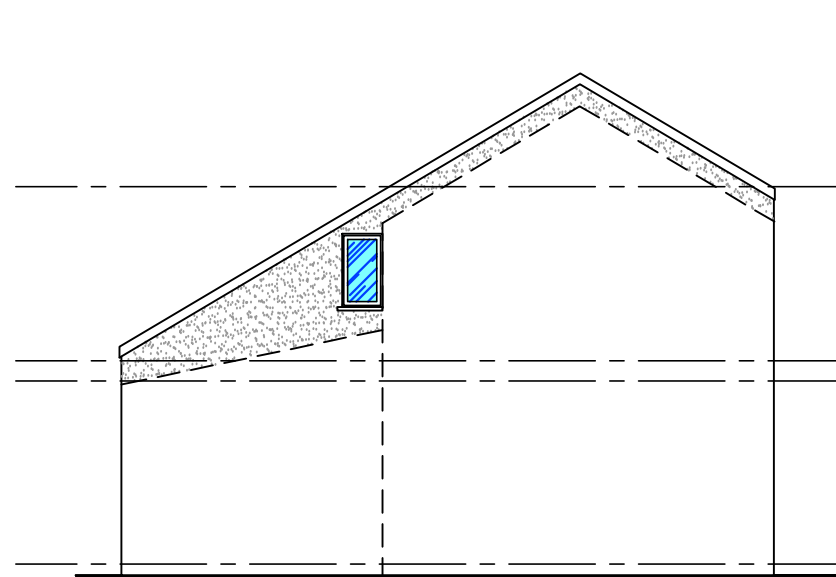
SIDE ELEVATION PRIOR TO WORKS
