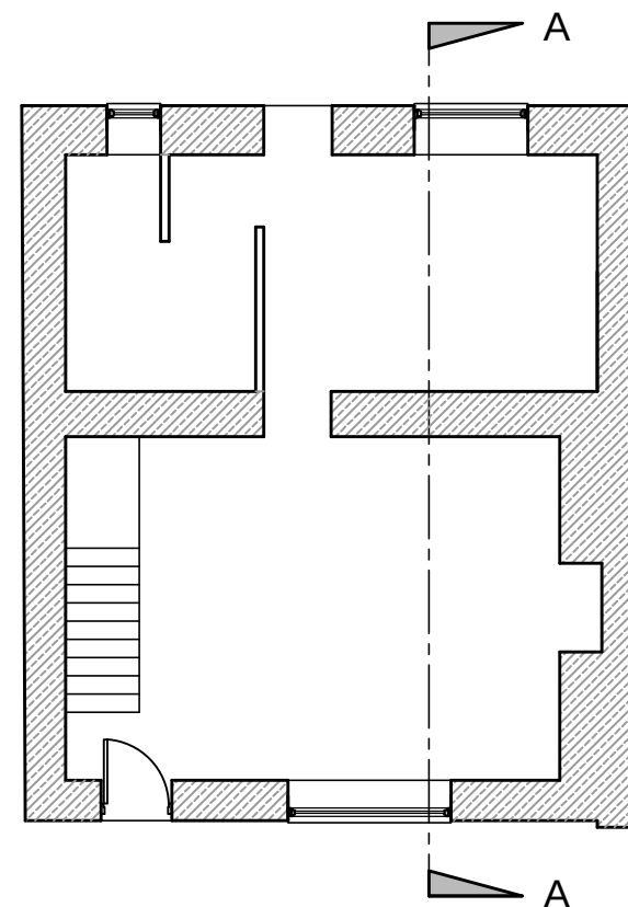
GROUND FLOOR PLAN PRIOR TO WORKS
