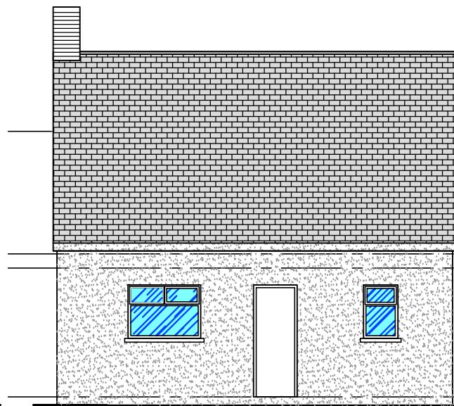
REAR ELEVATION PRIOR TO WORKS
