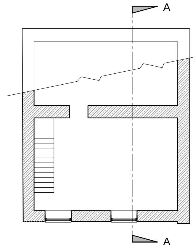
FIRST FLOOR PLAN PRIOR TO WORKS
