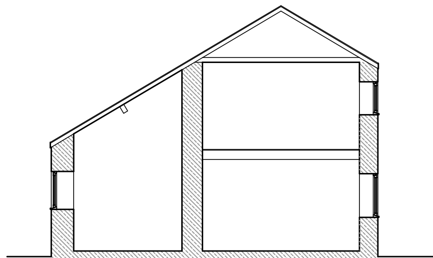
SECTION A-A PRIOR TO WORKS
