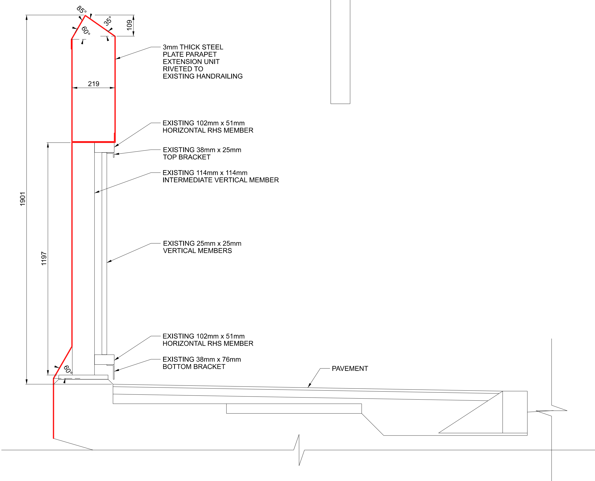
SECTION B - B
