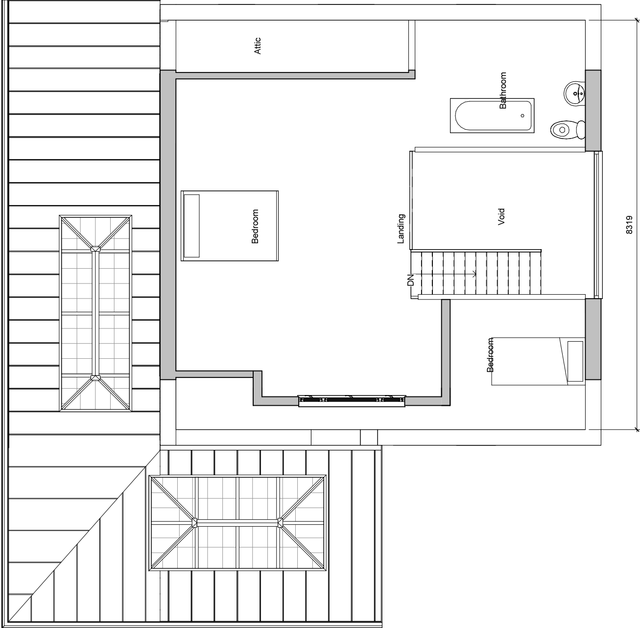
1 Proposed First Floor 1 : 50
