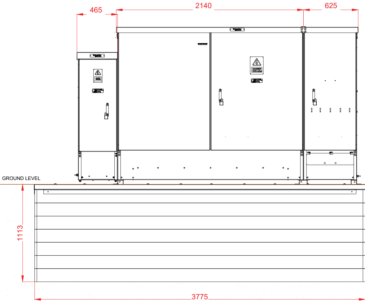
FRONT ELEVATION
