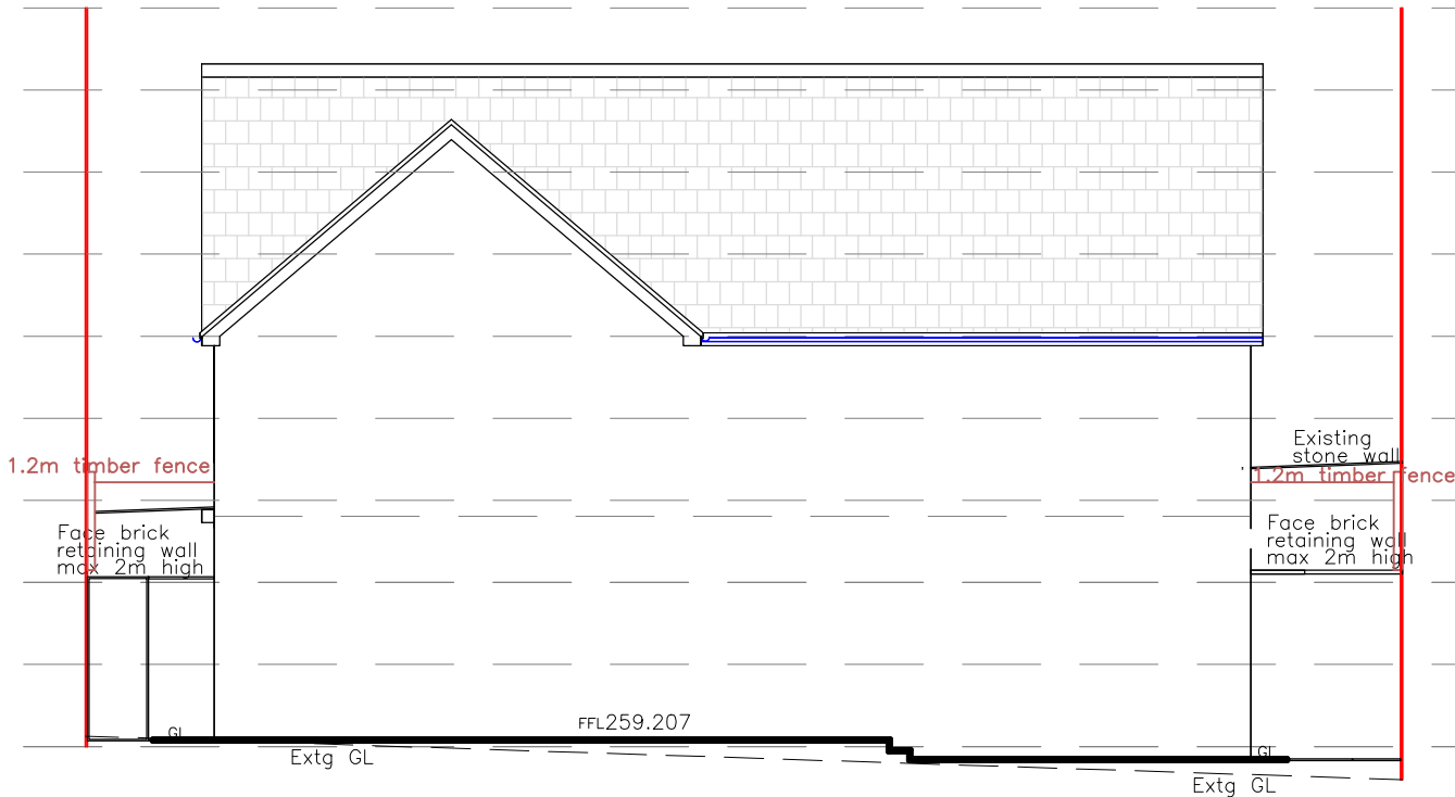
Proposed Site Section E-E 1:100
