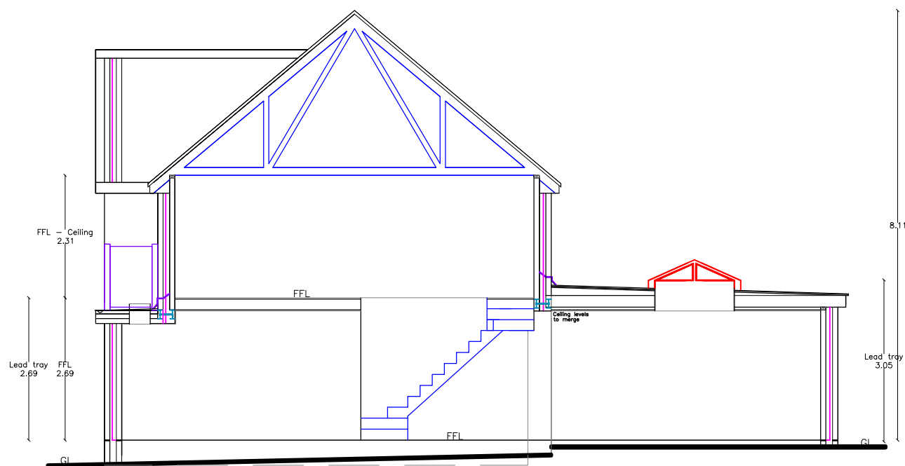
Proposed Section 1:100
