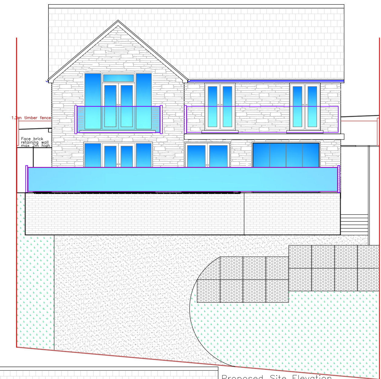
Proposed Site Elevation 1:100
