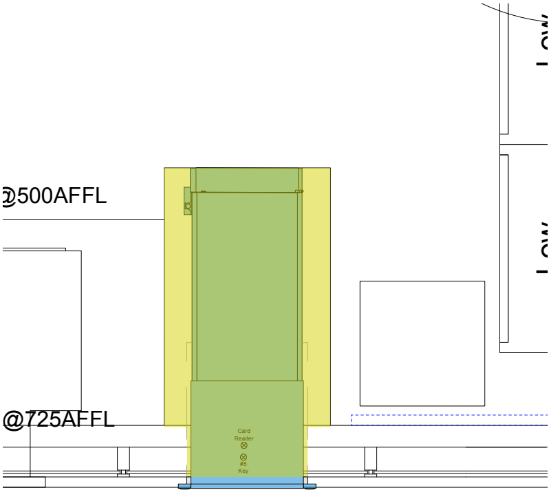
01 Detailed Plan Of Affected Area 1:25@A3
