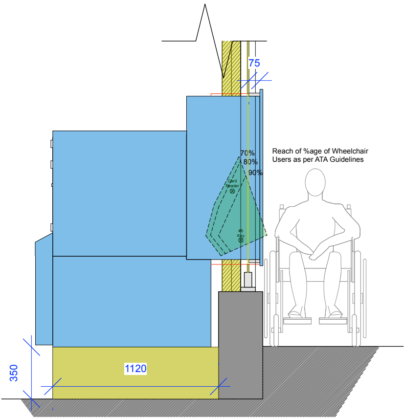
04 Detailed Section Of Affected Area 1:25@A3
