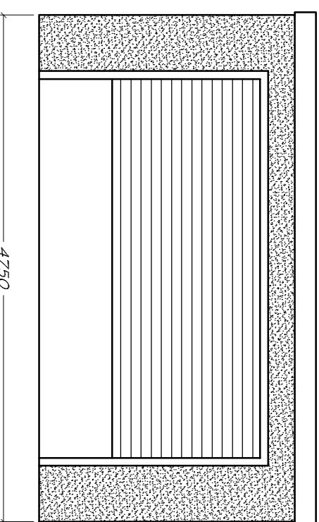
PROPOSED FRONT 1:50
