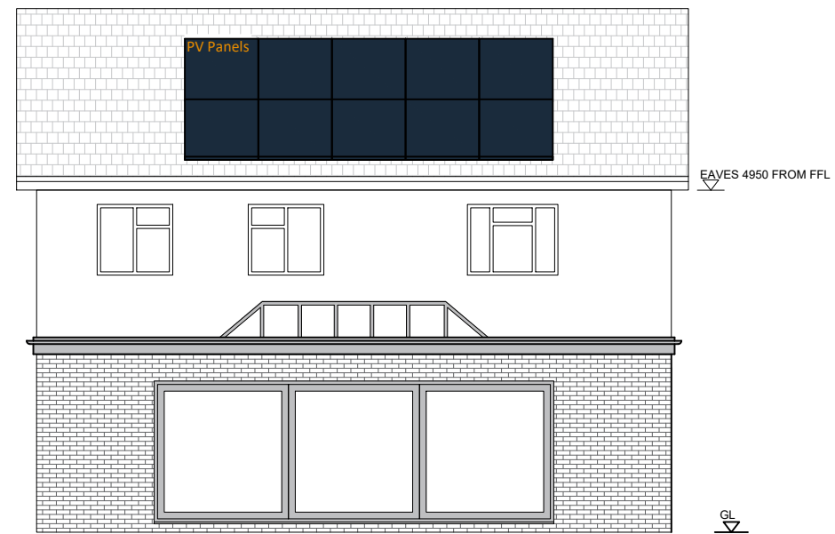
REAR ELEVATION
