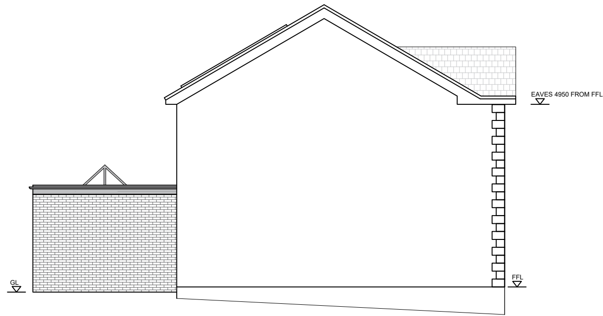
LEFT ELEVATION
