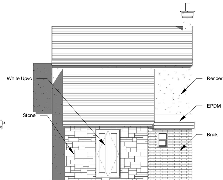
4 Proposed Rear Elevation 1 : 100
