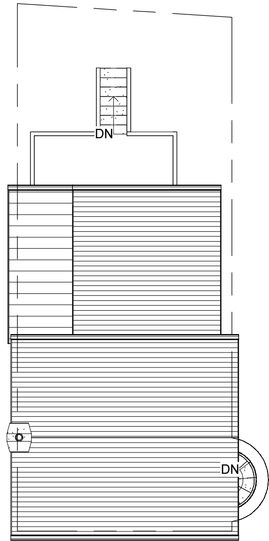
7 Proposed Site 1 : 100
