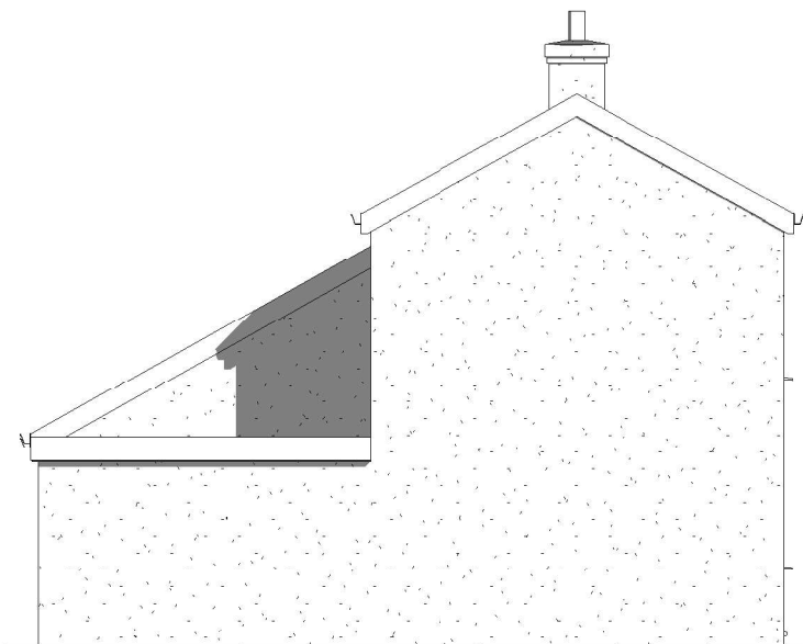
5 Proposed Side 1 Elevation 1 : 100
