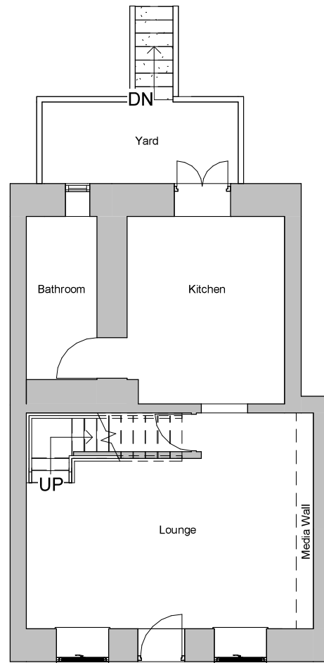
1 Proposed Ground Floor 1 : 100
