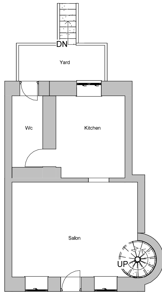
1 Existing Ground Floor 1 : 100
