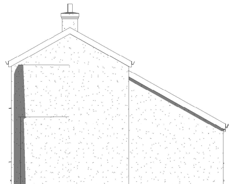
6 Existing Side 2 Elevation 1 : 100
